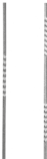
Art.20/01 Art.20/03 H 900 mm H 900 mm 12 x 12 mm 12 x 12 mm
